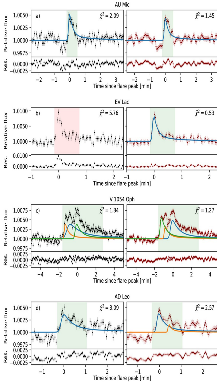
Example of some lightcurves of flaring stars obtained by ground and space based telescopes.
